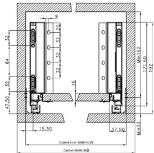
Slide Installation Spec. - High
