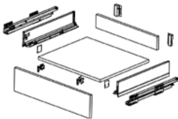
Double-Wall Drawer Low (accessories)
