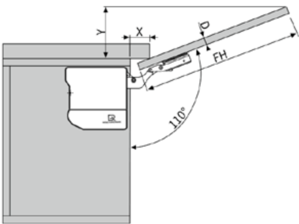
Space For Top Side Panel
