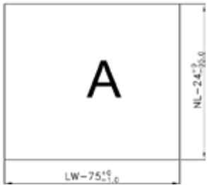
Bottom Panel T=16MM
