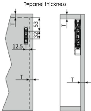
Space For Top Side Panel
