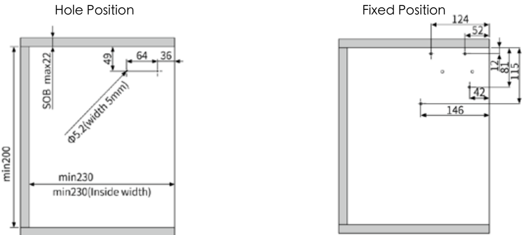
Panel Installation Size
