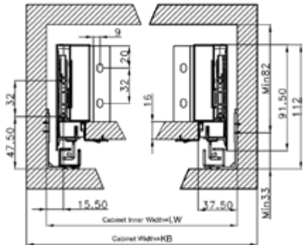
Slide Installation Spec. - Low
