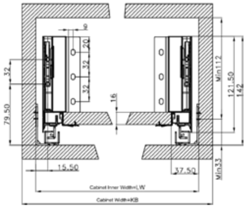
Slide Installation Spec. - Medium
